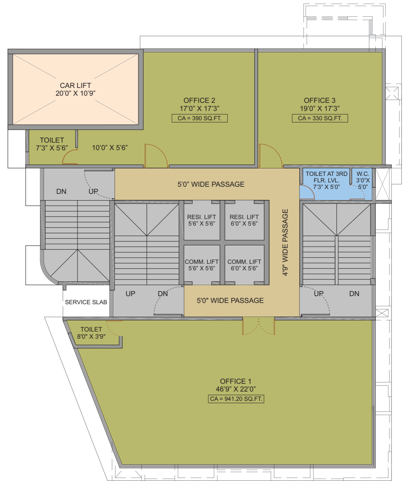
1st and 3rd Floor Plan
